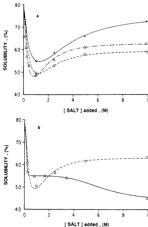
Figure 1. Salt-induced solubility profile of native soy isolate. (a) Key: O, solubility data for NaCl or \text{NH}_4\text{Cl} ; ---, theoretical curve for NaCl or \text{NH}_4\text{Cl} data; \Delta , solubility data for \text{NH}_4\text{Br} ; ---, theoretical curve for \text{NH}_4\text{Br} data; +, solubility data for NaI; ---, theoretical curve for NaI data. (b) Key: O, solubility data for \text{NH}_4\text{NO}_3 ; ---, theoretical curve for \text{NH}_4\text{NO}_3 data; \Delta , solubility data in (\text{NH}_4)_2\text{SO}_4 or \text{Na}_2\text{SO}_4 ; ---, theoretical curve for (\text{NH}_4)_2\text{SO}_4 or \text{Na}_2\text{SO}_4 data.
