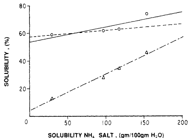
Figure 3. Salting-in solubilities ( S_2 from Tables I and II) versus literature solubilities of ammonium salts with corresponding anions (Wagman, 1968) of \text{Cl}^- , \text{Br}^- , \text{NO}_3^- , and \text{I}^- (left to right). Key: O, native soy isolate; —, least squares straight line for first three points only; ---, least squares straight line for all four points; \Delta , denatured soy isolate; ···, least-squares straight line for denatured soy isolate data.
